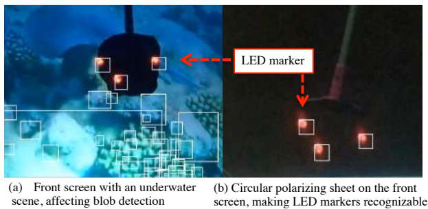
Figure 6: Background image stabilization for LED tracking.
